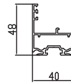
Khung bao 44
