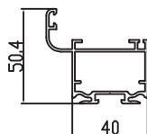
Khung bao 45
