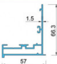
XFA-GK1305 T=1.5mm W=0.94 Kg/m
