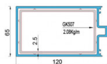
XFA-GK501 T=2.5mm W=2.70 Kg/m
