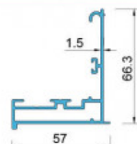
XFA-GK1275 T=1.5mm W=0.97 Kg/m
