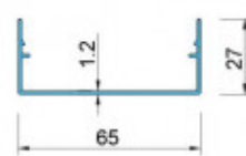
XFA-GK066 T=1.2mm W=0.40 Kg/m
