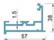
XFA-GK1365 T=1.5mm W=0.80 Kg/m
