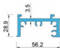
XFA-GK865 T=3.5mm W=1.21 Kg/m
