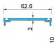
XFA-GK015 T=3.0mm W=0.57 Kg/m
