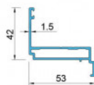
XFA-GK1315 T=1.5mm W=0.72 Kg/m
