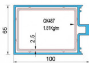
XFA-GK481 T=2.5mm W=2.42 Kg/m
