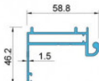
XFA-GK1255 T=1.5mm W=0.91 Kg/m
