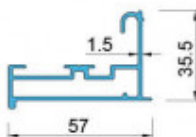
XFA-GK1325 T=1.5mm W=0.79 Kg/m
