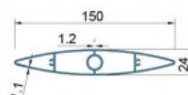
XFA-H25X100 T=0.9mm W=0.598 Kg/m
