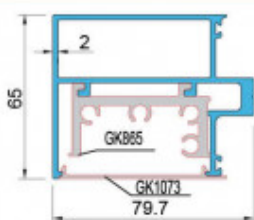
XFA-GK993 T=2.0mm W=1.90 Kg/m
