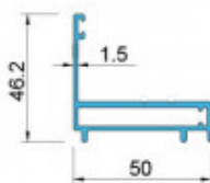
XFA-GK1295 T=1.5mm W=0.75 Kg/m
